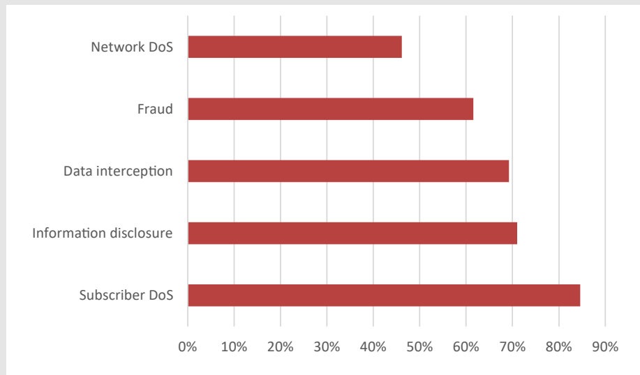
Pic. 2 – Success rate of executed attacks
